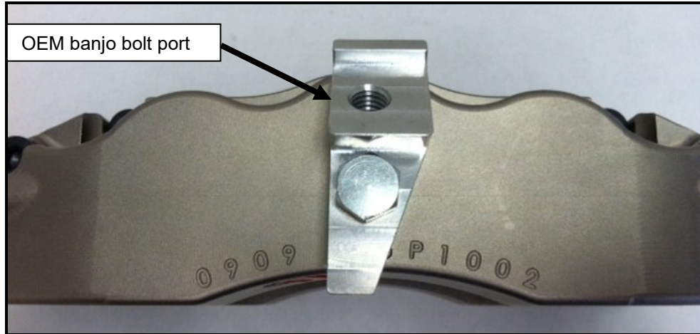
Figure 6: (96-04 models) Hose adaptor installed (driver's side) to allow use of original hoses. Orient adaptor to desired position for hose fitment
