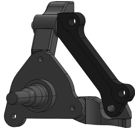
Figure 3. Intermediate bracket installed (outboard view)
