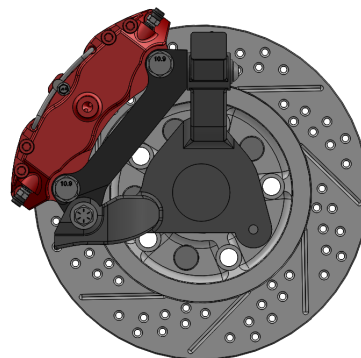
Figure 7. Caliper assembly installed
