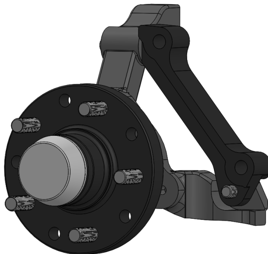
Figure 5. Cotter pin and dust cap installed
