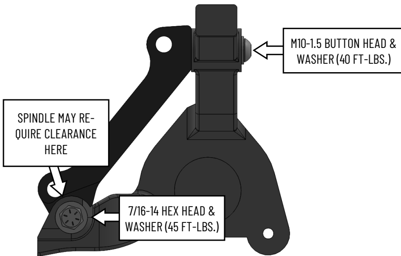
Figure 2. Intermediate bracket installed (inboard view)
