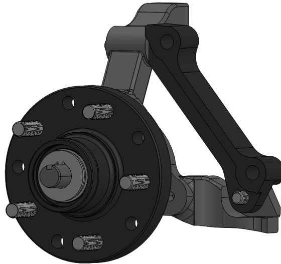
Figure 4. Wheel hub assembly installed
