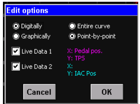
Figure 43 – Edit Options
