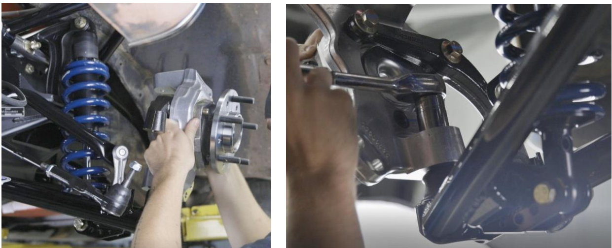
Figure 93 - Install Spindle on Lower Control Arm
