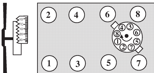
Figure 3 1-8-4-3-6-5-7-2 Chrysler 318-340-36- c.i.d. Turn distributor counter-clockwise to advance timing
