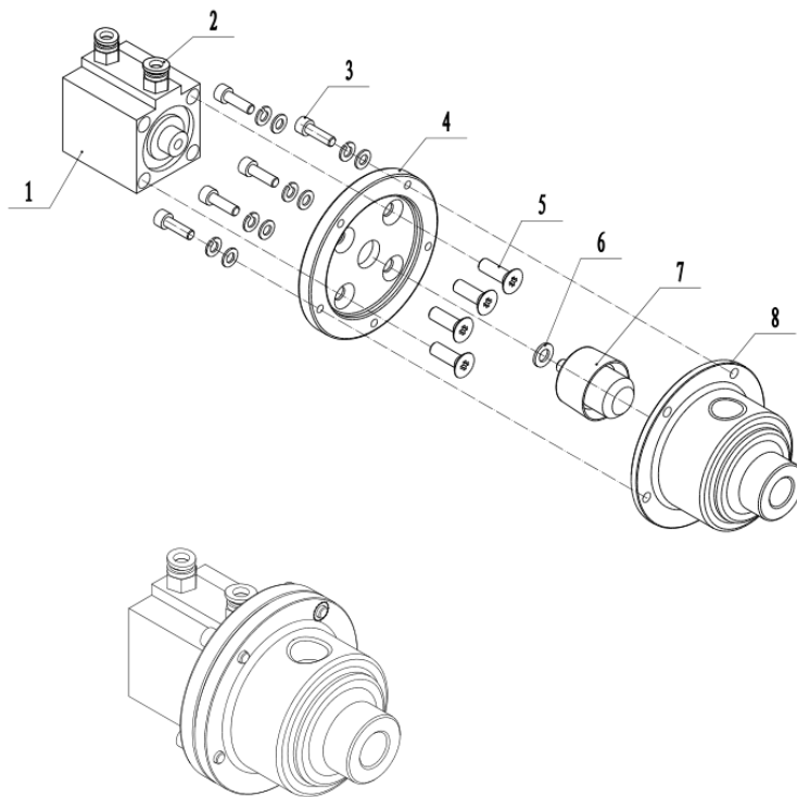
42059 – Hose adapter
