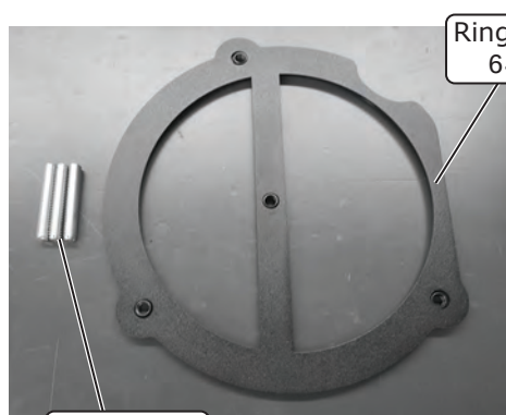
(3) 1/4-20 Full-Length Studs
