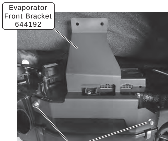
Engine Compartment View
