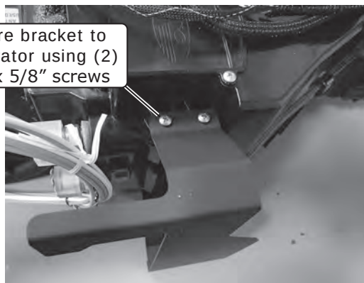
Top View of Module
