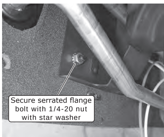
Passenger Compartment View
