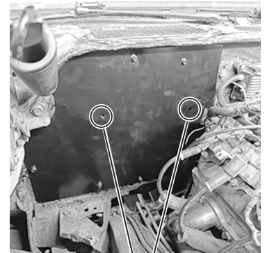
Using full-length studs locate upper mounting holes in firewall
