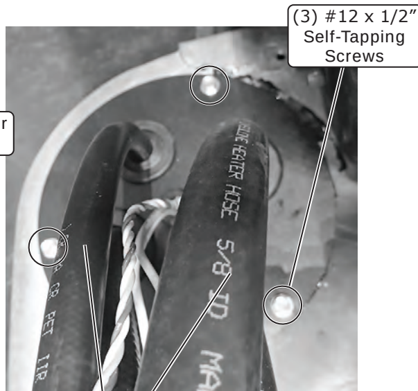
Route A/C and heater hoses through fresh air cover
