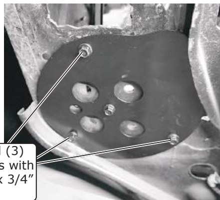
Engine Compartment View
