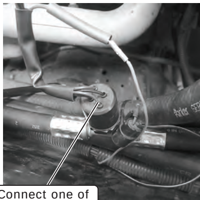
Connect one of blue leads from trinary switch to gray wire from OEM A/C high-pressure fan switch wiring
