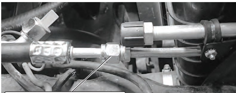
Install straight fitting of #6 A/C hose onto #6 drier hardline
