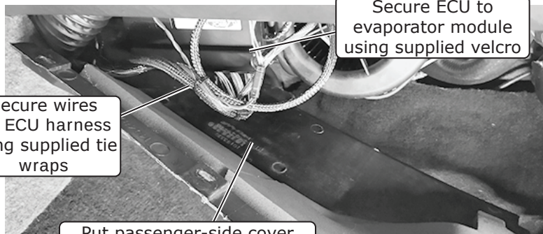
Put passenger-side cover plate into place in floorboard
