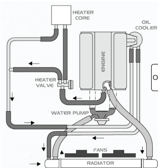
OEM Cooling System
