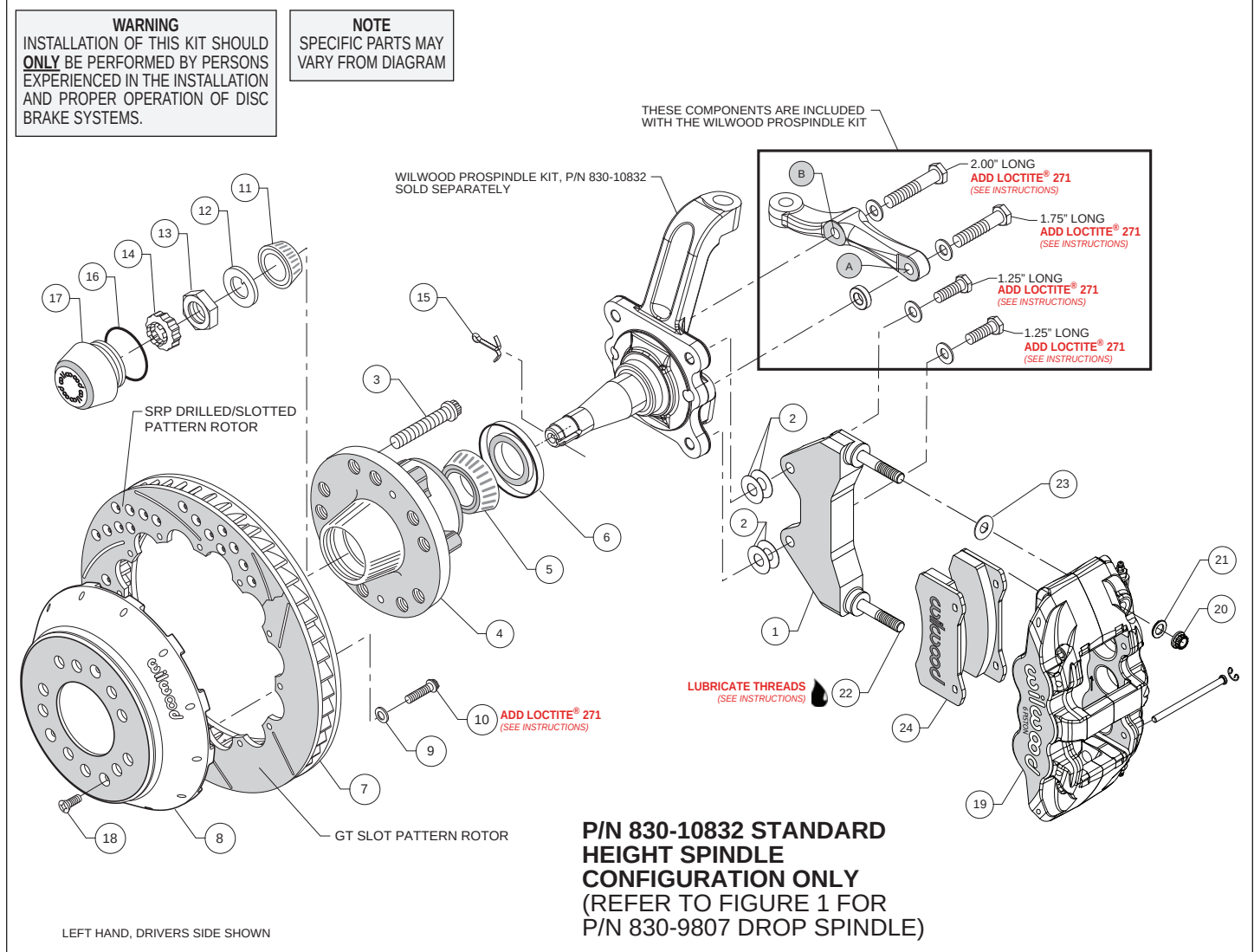
Figure 2. Installation Configuration For Standard Height Spindle, P/N 830-10832
