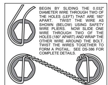
Figure 4. Safety Wire Diagram
