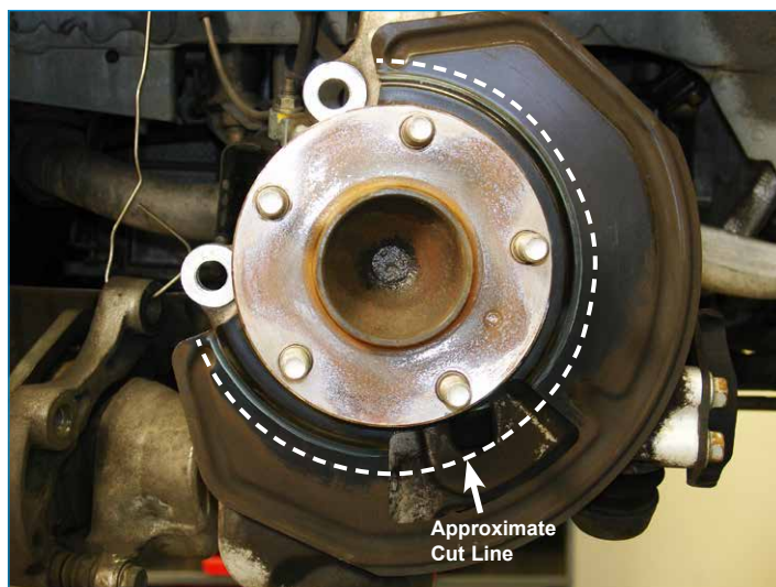
Photo 1. Dust Shield Modification
