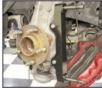
Photo 1 (Generic Axle Hub Shown)
