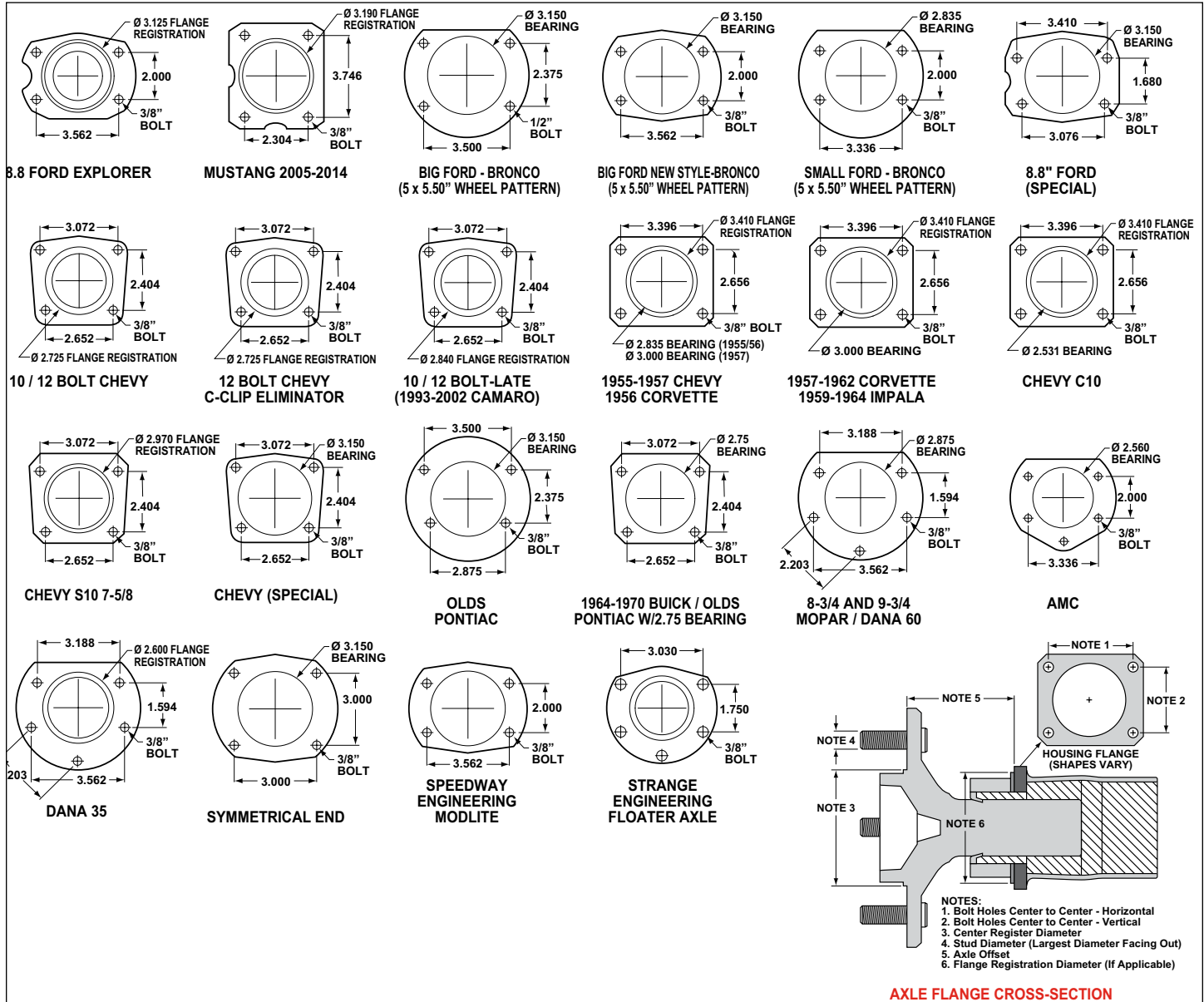
Figure 6. Rear Housing Flange Chart and Axle Flange / Offset Cross-Section
