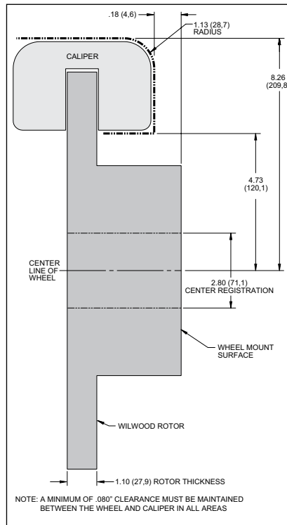
Figure 3A P/N 140-15846. Wheel Clearance Diagram
