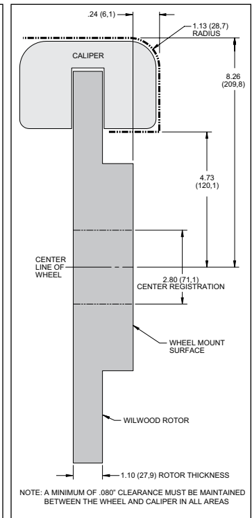
Figure 3B P/N 140-16170. Wheel Clearance Diagram
