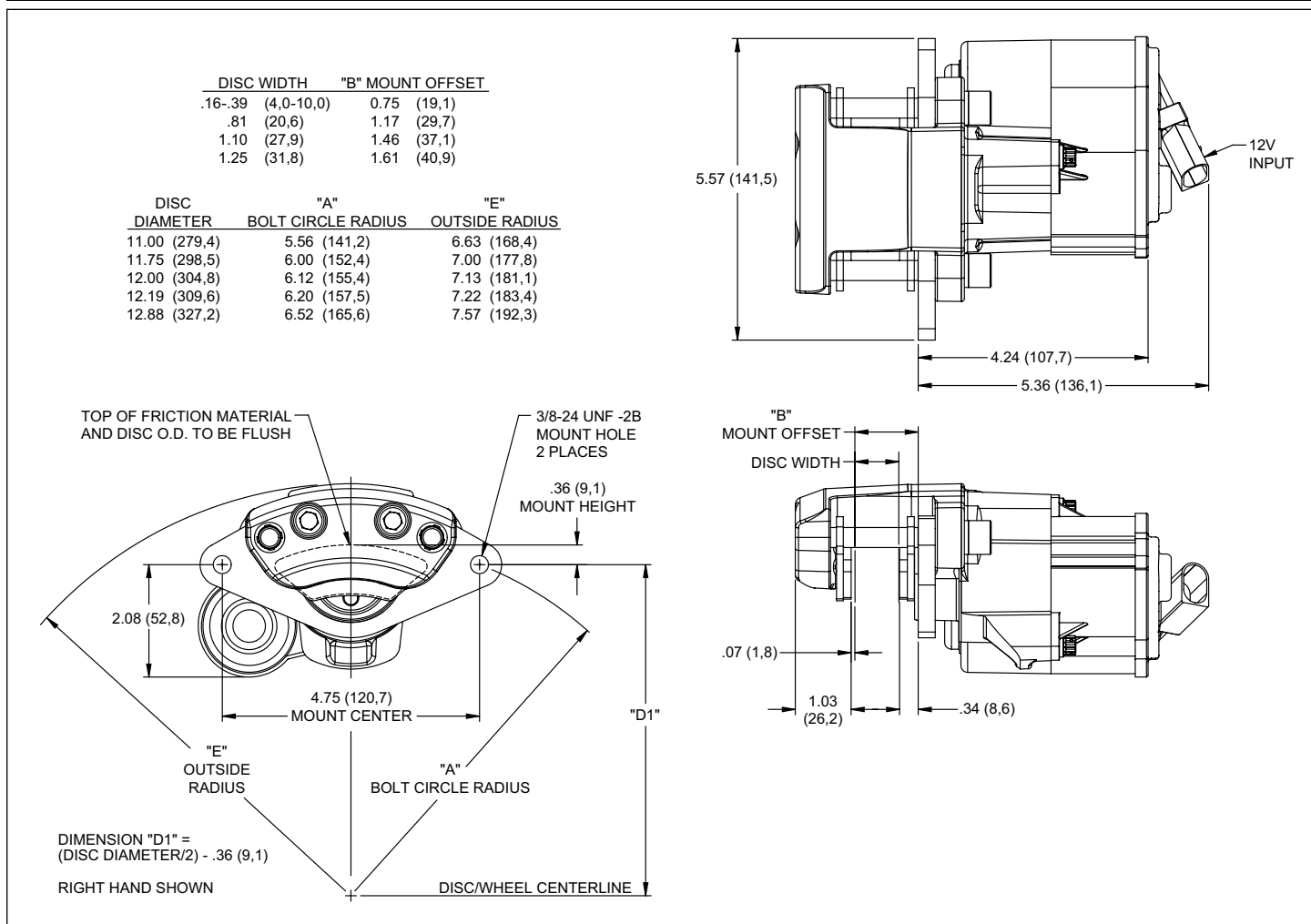
Figure 3. EPB Caliper
