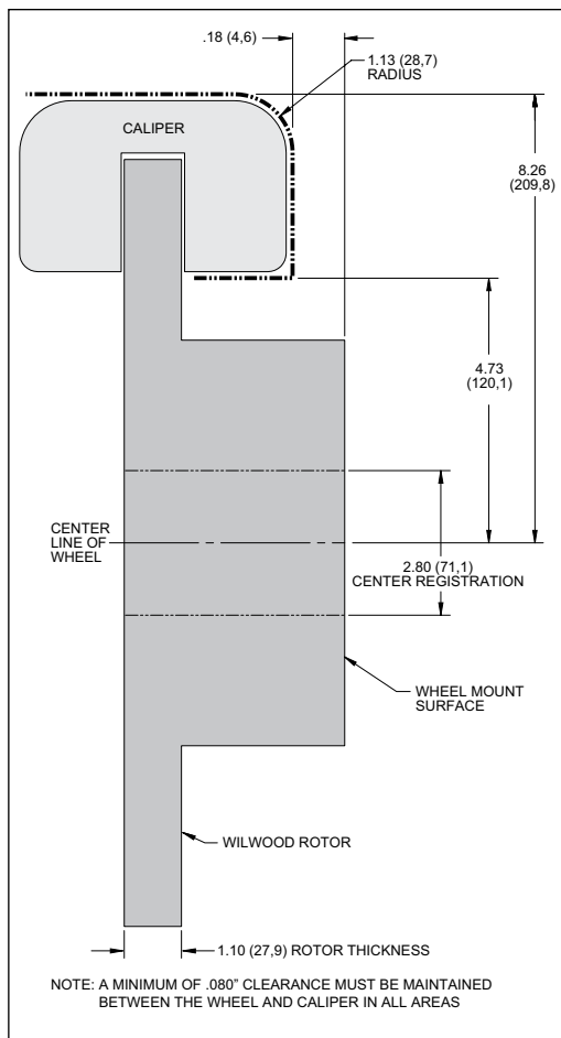
Figure 3. Wheel Clearance Diagram
