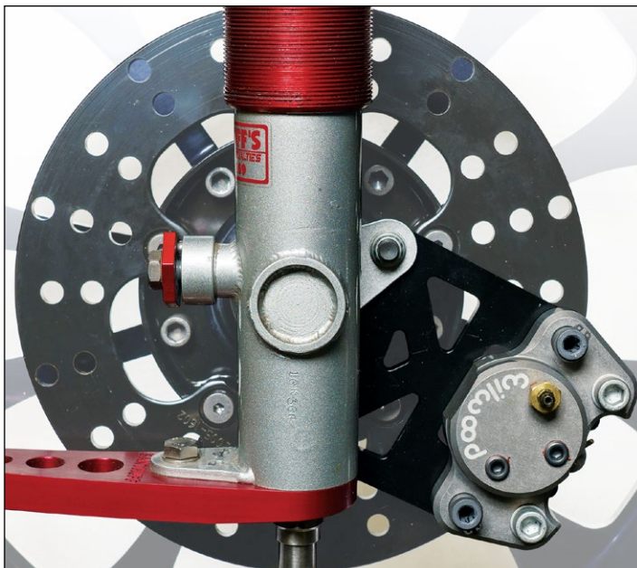
Photo 10 - Santhuff's strut
