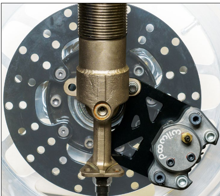
Photo 9 - Afco strut
