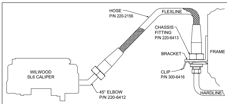
Figure 4. Brake Line Diagram
