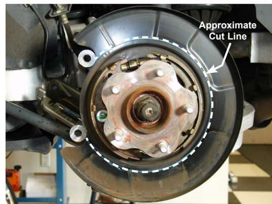
Photo 1. Dust Shield/Backing Plate Modifications
