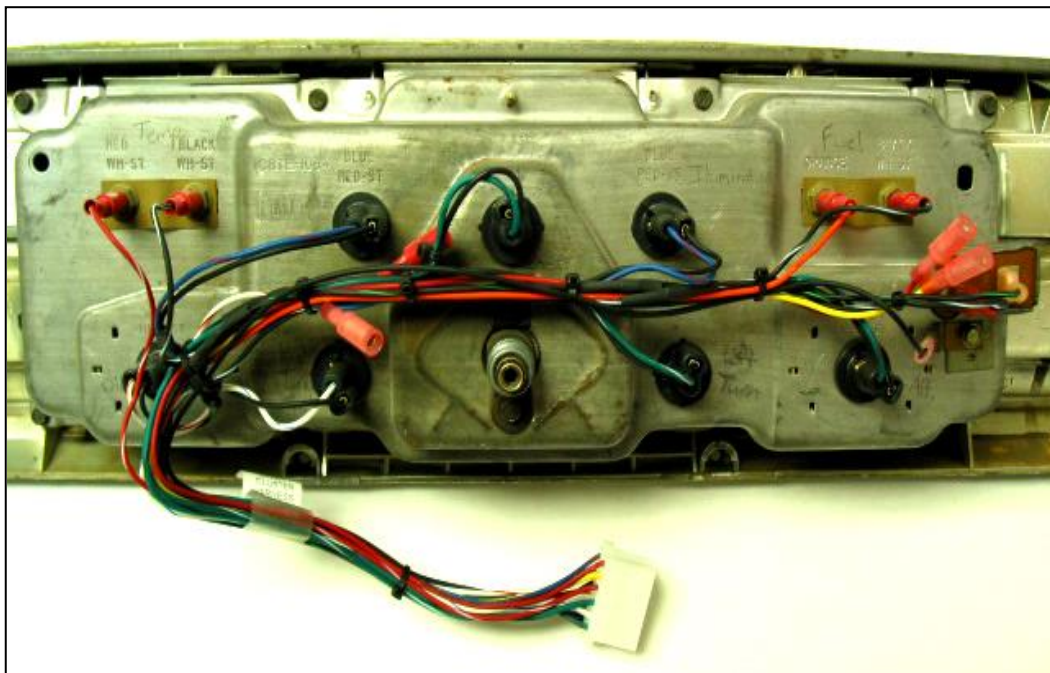
Figure 7-34 1967 thru 1969 Models - Cluster Harness
