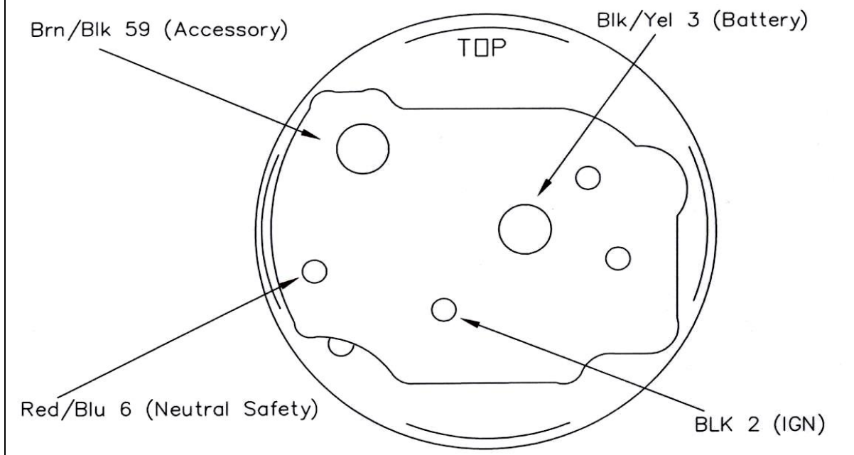
1968 – 1970 Ford Truck Ignition Switch
