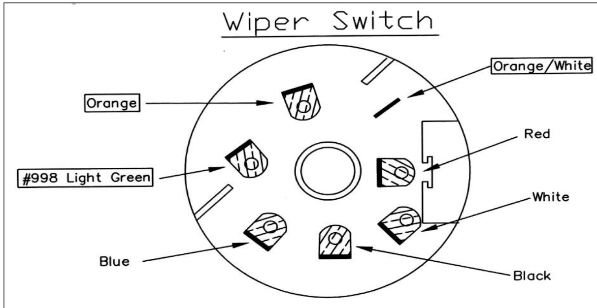
Figure 7-20 Wiper Switch Connections (All Models)
