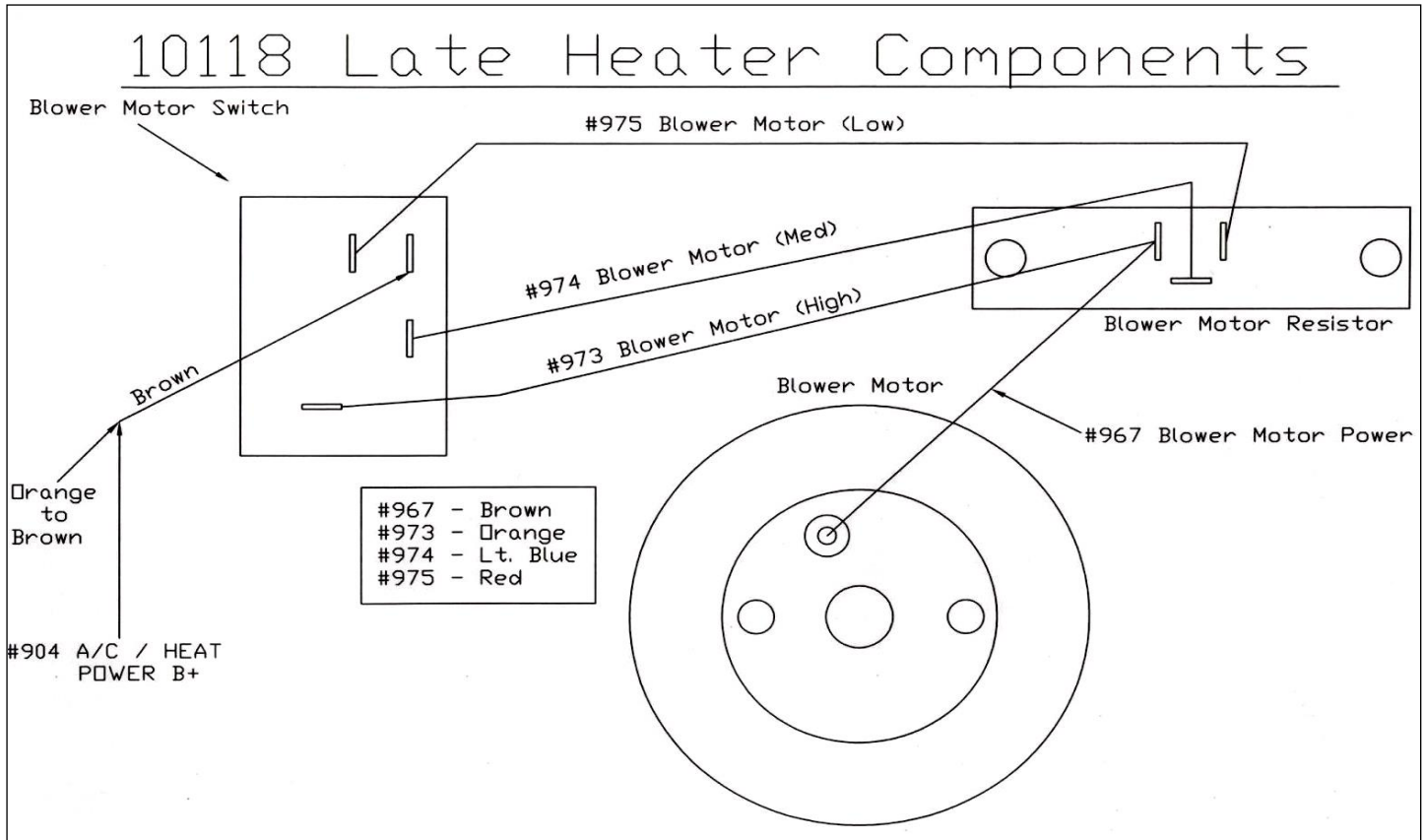
Figure 7-30 Heater Harness Installation for 1973-1977 years only.
