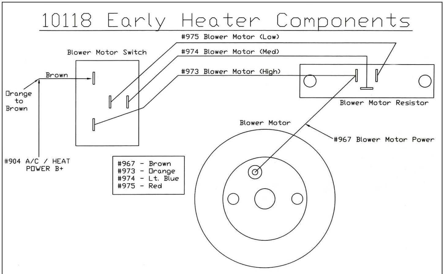
Figure 7-28 Heater Harness Installation for 1967-1972 years only.
