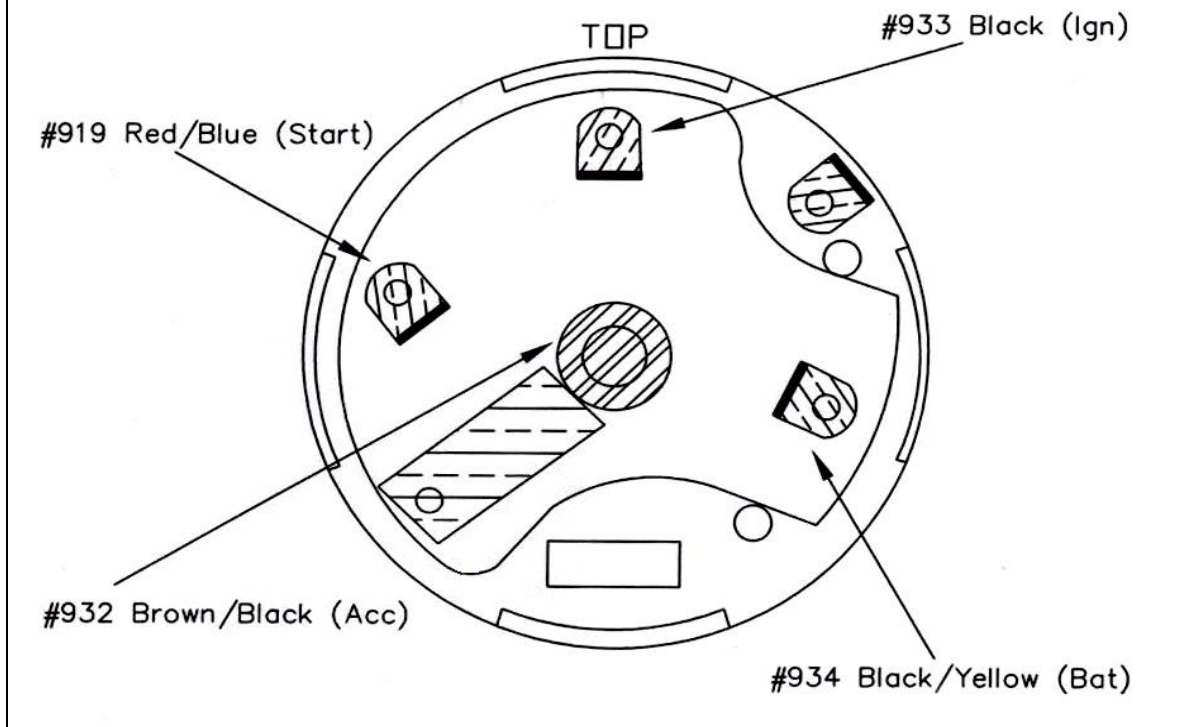
1967 Ford Truck Ignition Switch
