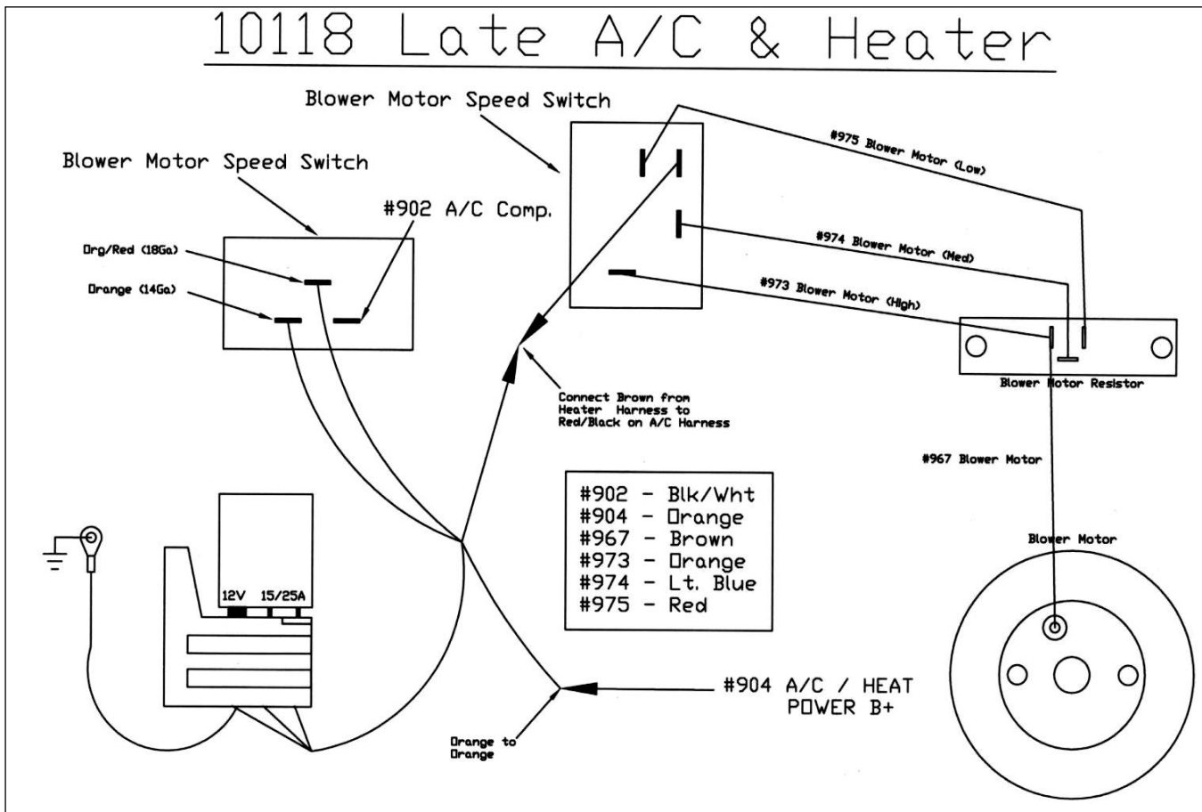
Figure 7-31 A/C - Heater Harness Installation for 1973-1977 years only
