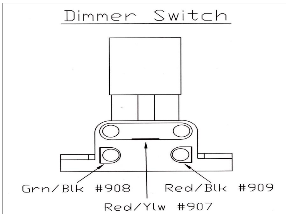
Figure 7-22 Routing the Dimmer Switch Wires
