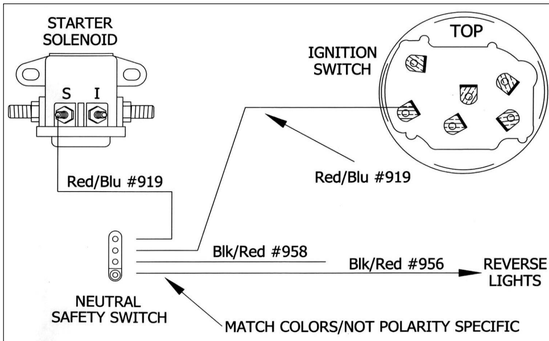
Figure 7-10 NEUTRAL SAFETY SWITCH (All Models with Auto Trans)
