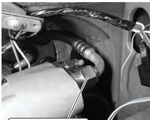
Install 90° fitting on #10 compressor/ evaporator A/C hose onto #10 fitting on block valve adapter
