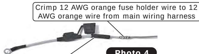
Install heat shrink over 12 AWG orange standard fuse holder assembly wire
