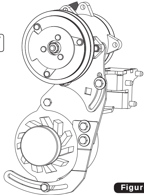
Finished Assembly, Front View
