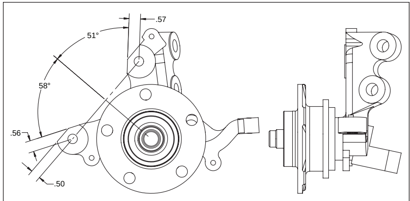
Figure 3. Spindle Modifications
