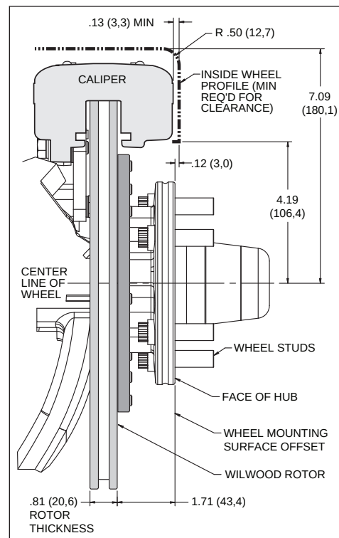
Figure 3. Wheel Clearance Diagram
